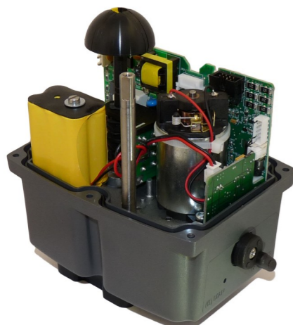
With battery failsafe installed
